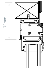
Head Detail
