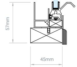
Cill Detail
