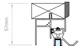
Head Detail
