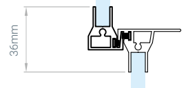
Cill Detail
